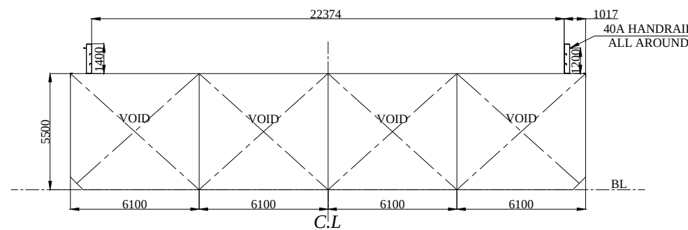
SECTION
