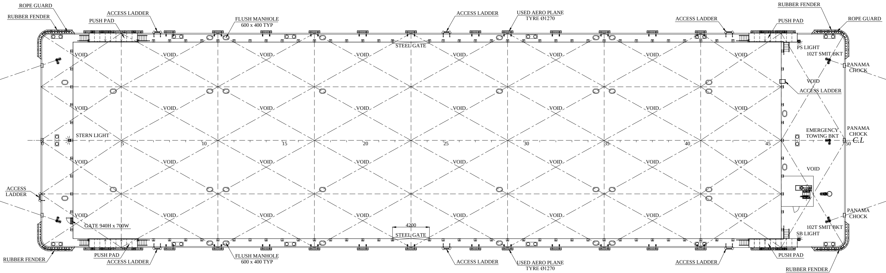
MAIN DECK PLAN
