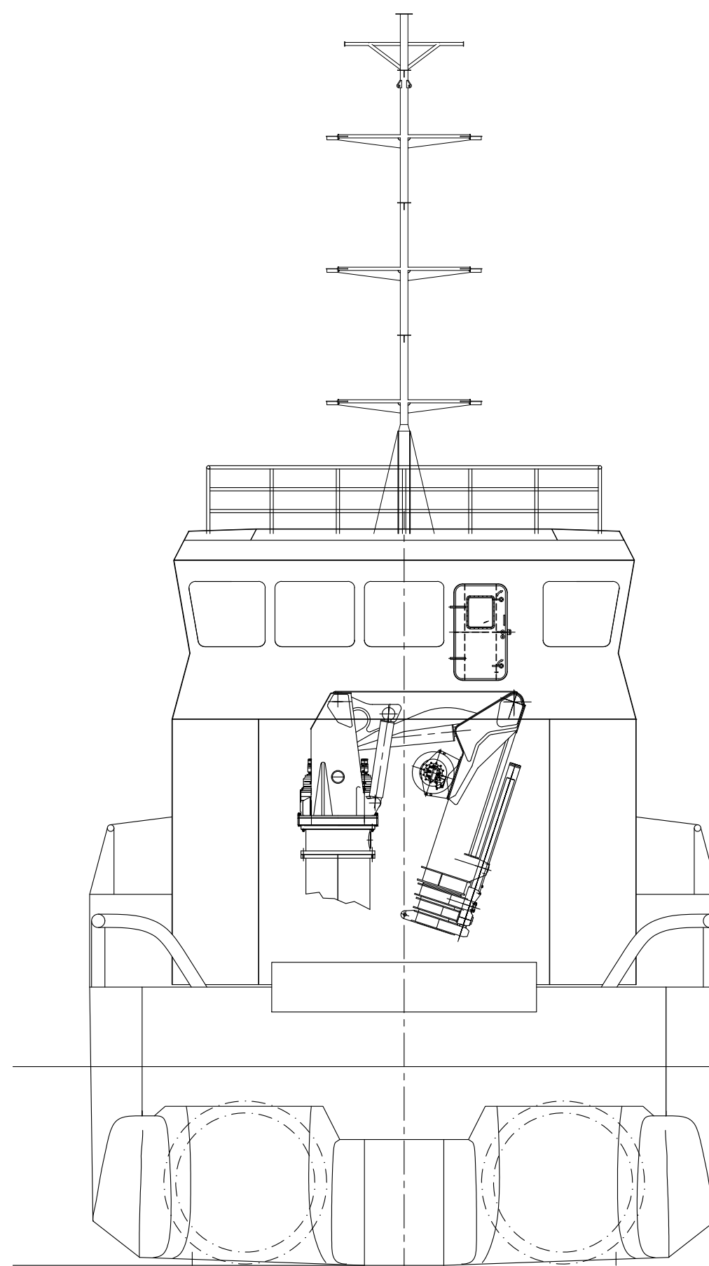
AFT VIEW
