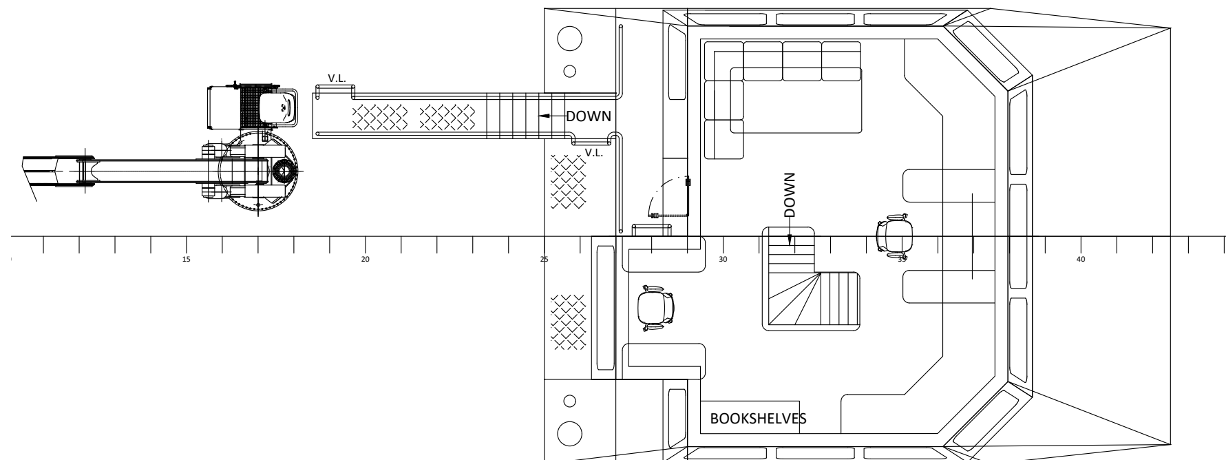
BRIDGE DECK PLAN
