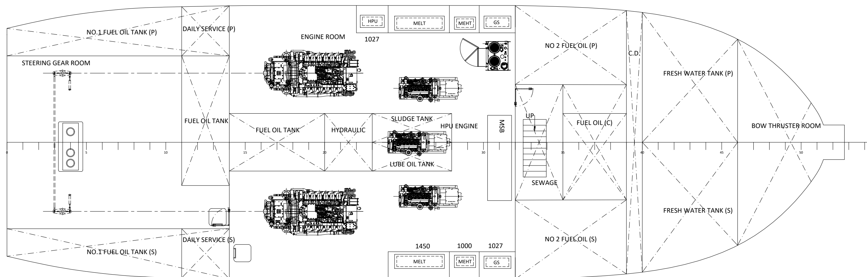
BELOW DECK PLAN
