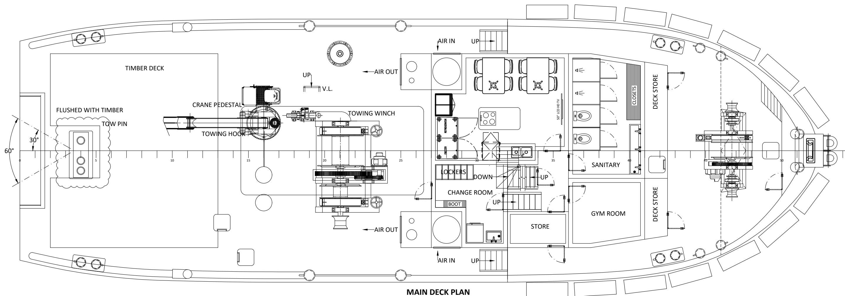
MAIN DECK PLAN
