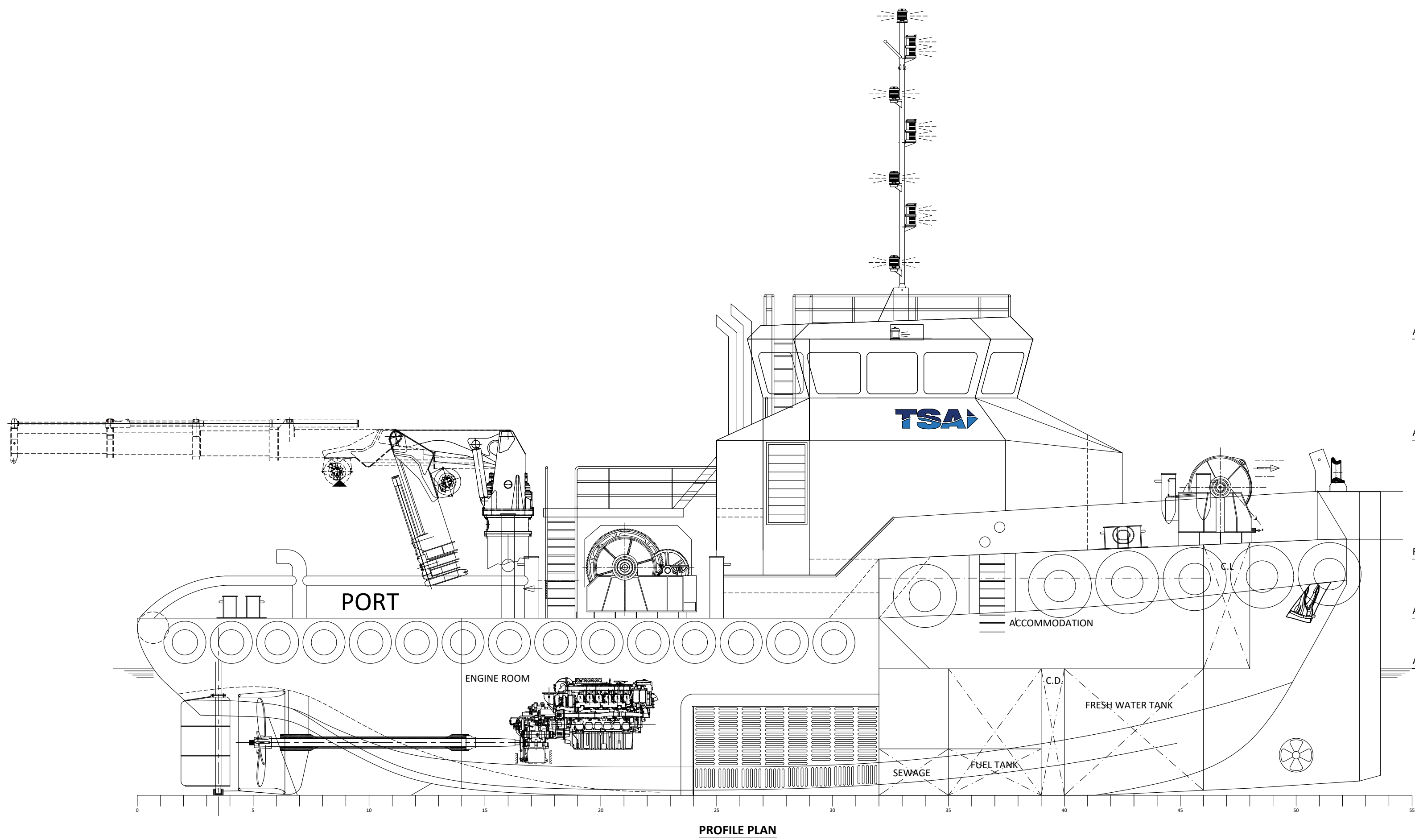
PROFILE PLAN
