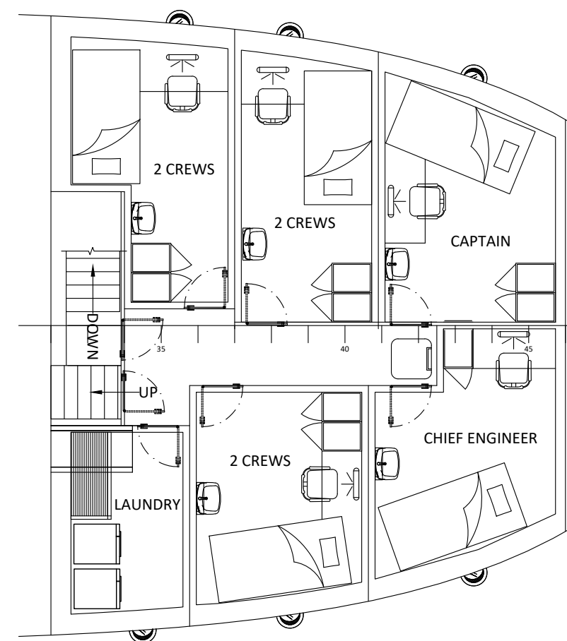
ACCOMMODATION DECK PLAN
